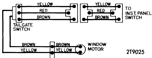
CHRYSLER CORP. TAILGATE WIRING DIAGRAM
