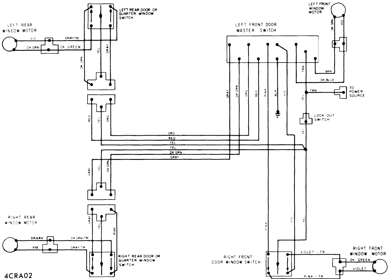
POWER WINDOW WIRING DIAGRAM CHRYSLER, IMPERIAL, MONACO & GRAN FURY SHOWN, OTHERS SIMILAR
