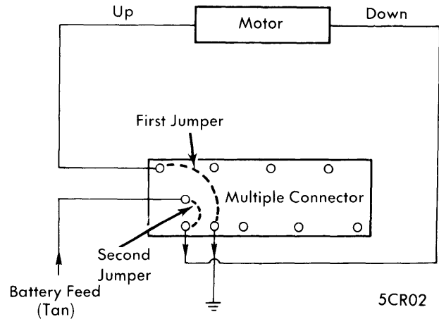
SWITCH "DOWN" TEST CIRCUIT
