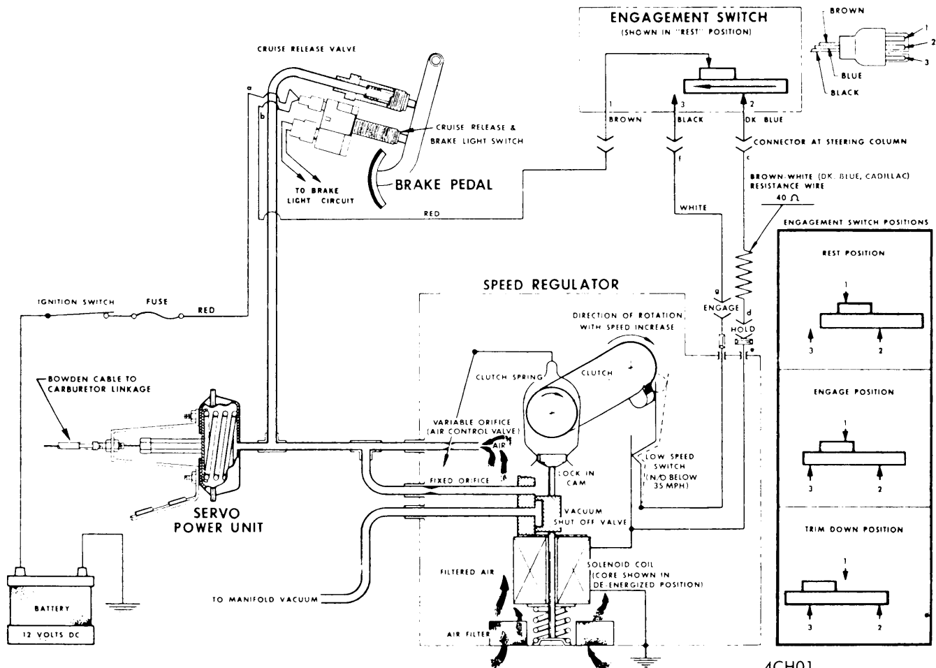
CHEVROLET VACUUM & ELECTRICAL DIAGRAM (OTHER MODEL SYSTEMS SIMILAR)
