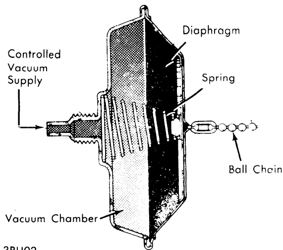
SERVO UNIT CROSS SECTION
