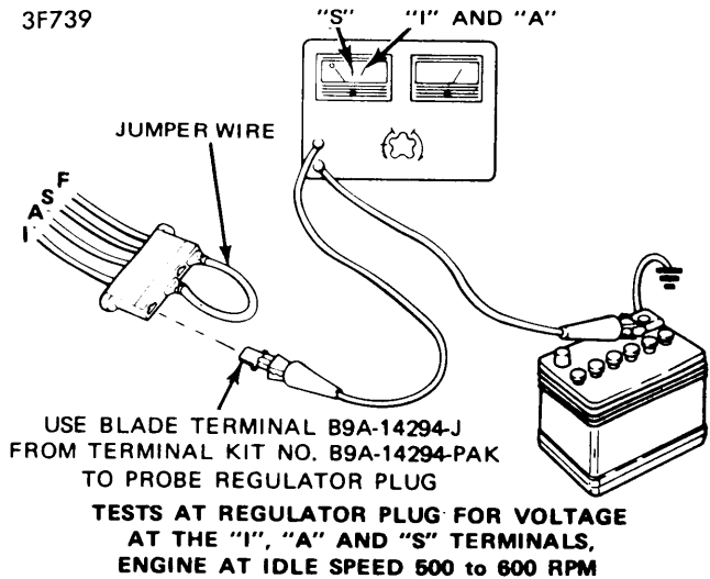
REGULATOR PLUG VOLTAGE TEST
