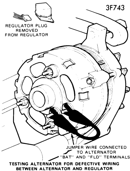
REAR TERMINAL JUMPER WIRE CONNECTION
