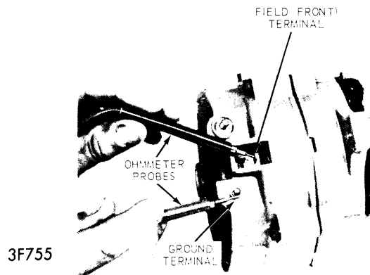
FIELD OPEN OR SHORT CIRCUIT TEST
