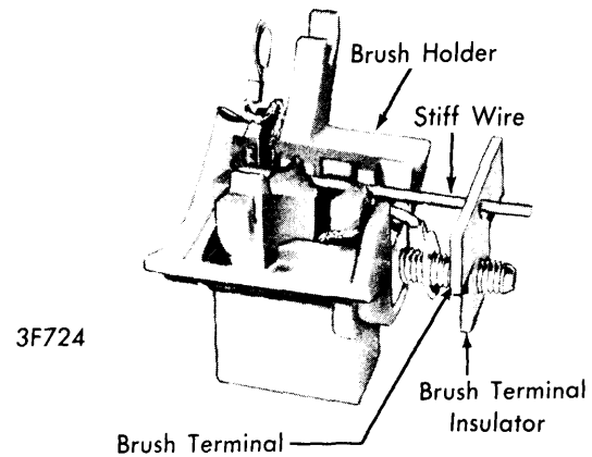
3F724 INSTALLING BRUSHES IN BRUSH HOLDER
