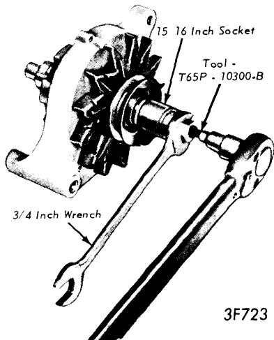
3F723 REMOVING ALTERNATOR PULLEY
