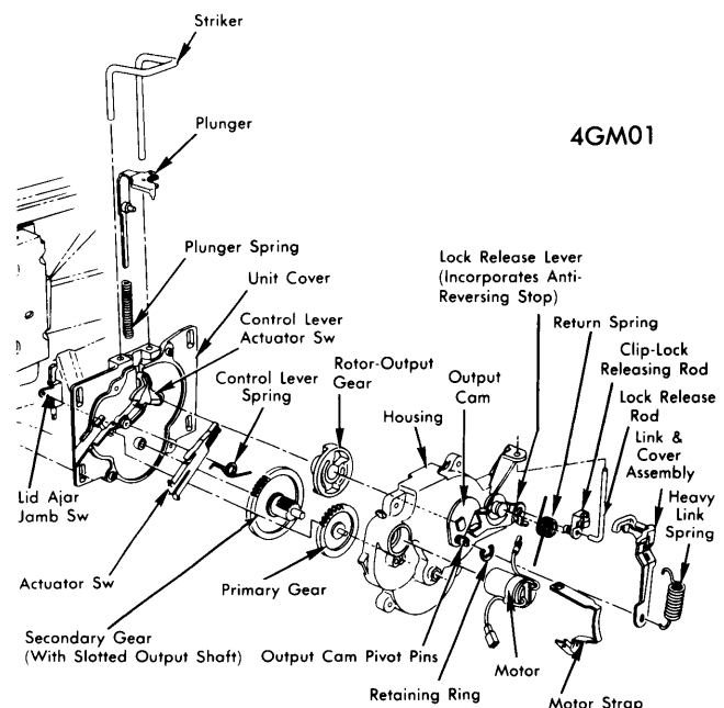
ELECTRIC CLOSING UNIT COMPONENTS
