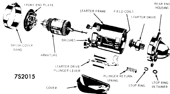
FORD MOTOR CO. POSITIVE ENGAGEMENT STARTER ASSEMBLY
