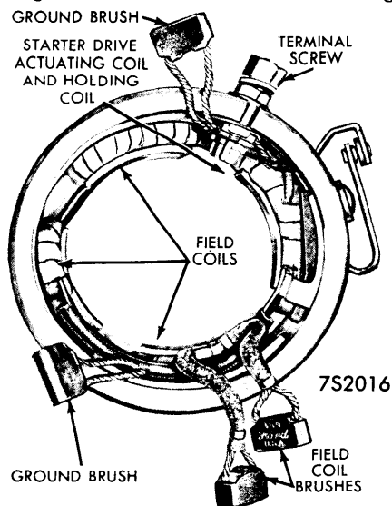
FIELD COIL ASSEMBLY
