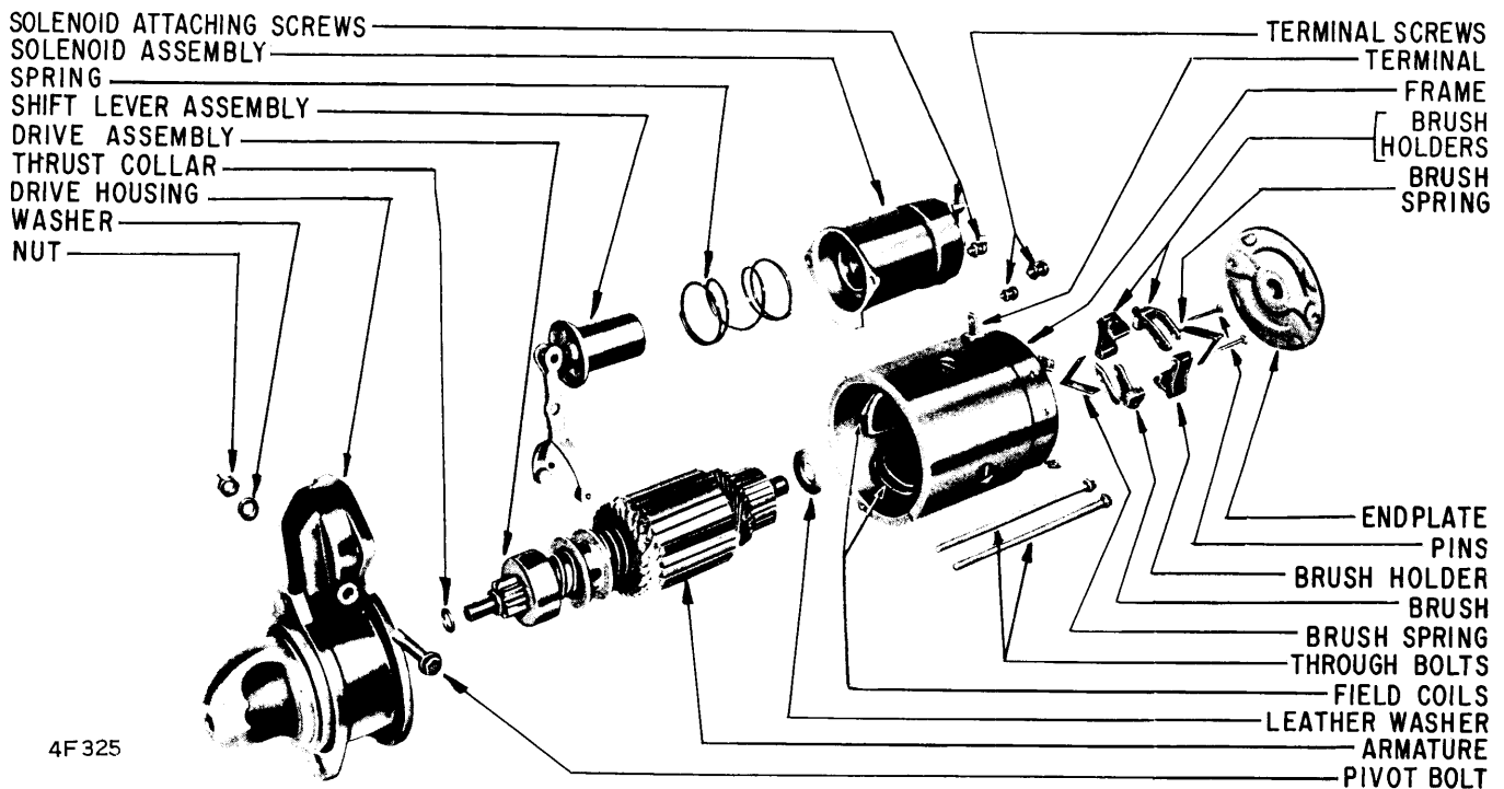
DELCO-REMY ENCLOSED HOUSING STARTER ASSEMBLY
