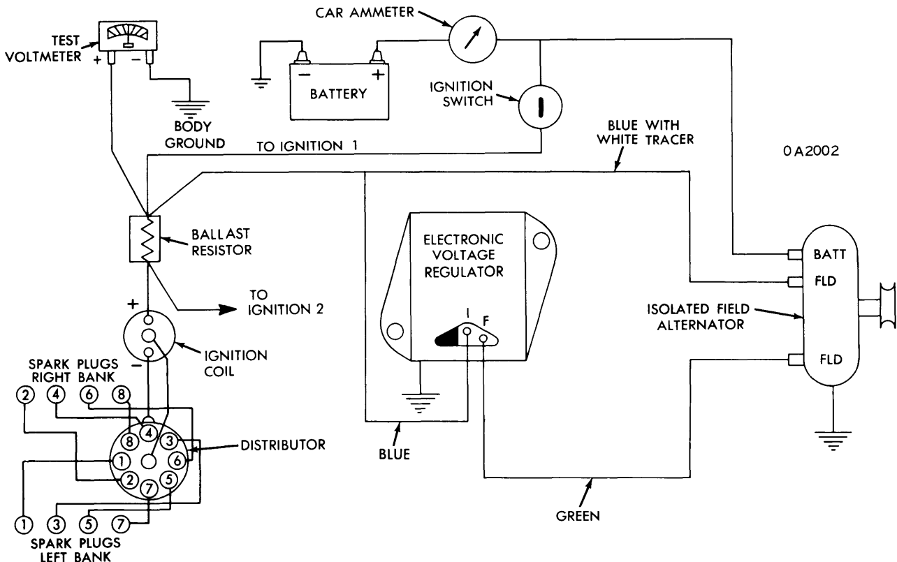
VOLTAGE REGULATOR TEST CONNECTIONS
