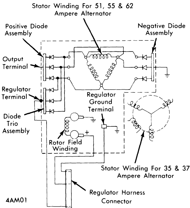
ALTERNATOR INTERNAL CIRCUITS
