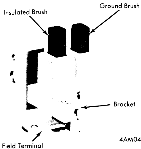
BRUSH ASSEMBLY
