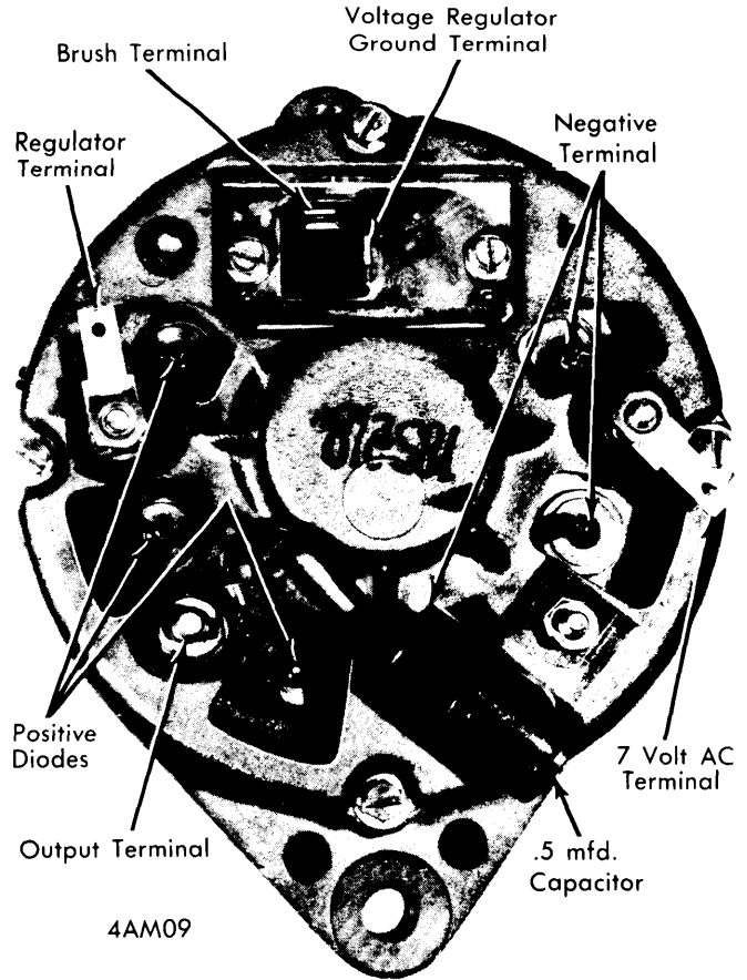
ALTERNATOR REAR VIEW
