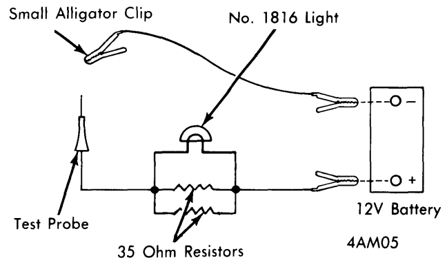
DIODE TRIO LOAD TEST
