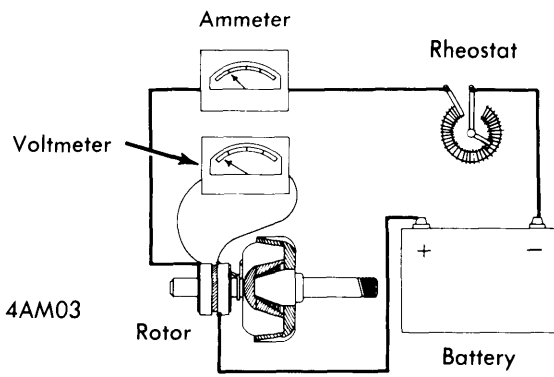
ROTOR CURRENT DRAW TEST
