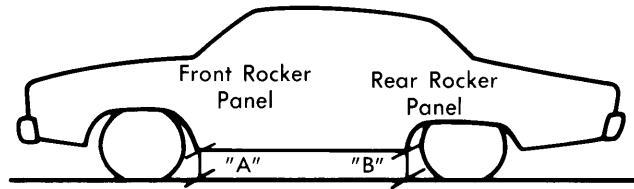
Fig. 1 Ride Height Measuring Points (All Models)
