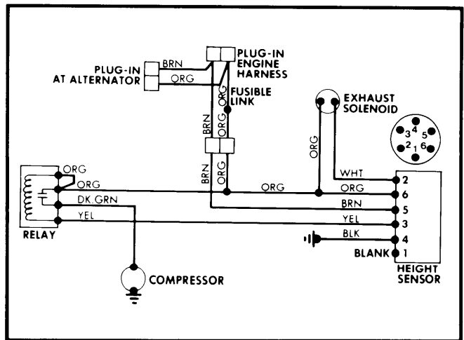
Fig. 9 Electronic Level Control Circuit Diagram (Buick, Exc. Riviera, and Pontiac)
