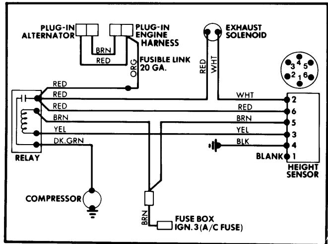
Fig. 8 Electronic Level Control Circuit Diagram (Oldsmobile, Exc. Toronado)
