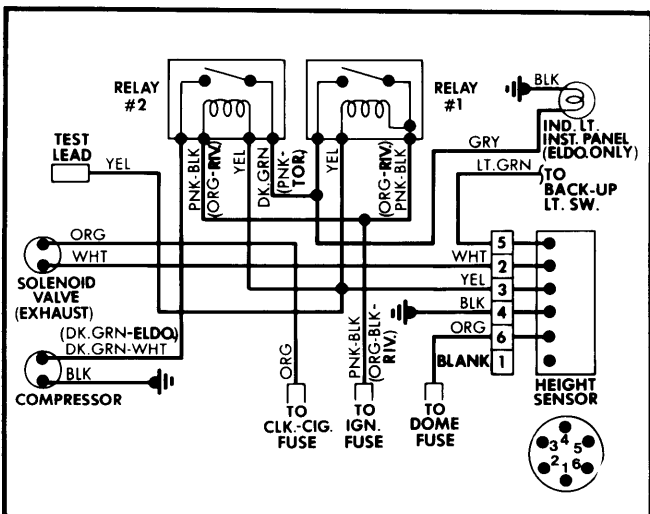
Fig. 7 Electronic Level Control Circuit Diagram (Eldorado, Riviera, Seville and Toronado)
