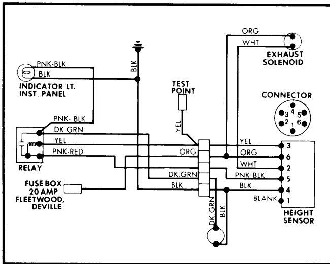
Fig. 6 Electronic Level Control Circuit Diagram (Cadillac, Exc. Eldorado and Seville)
