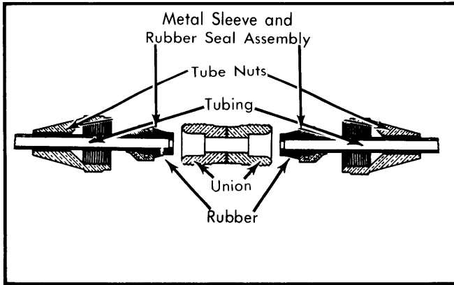
Fig. 5 Air Line Repair Coupling
