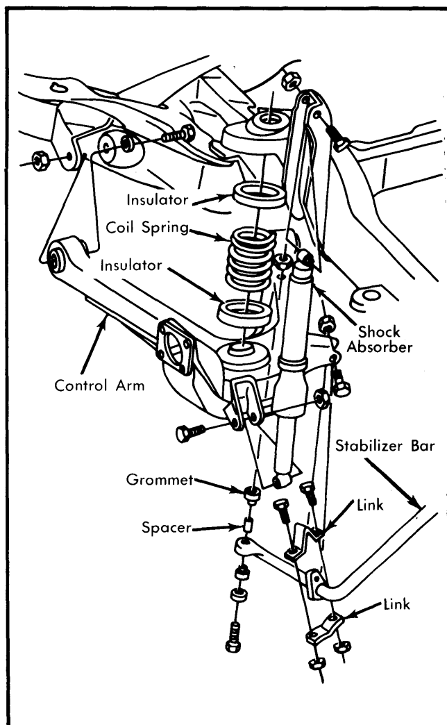
Fig. 1 Eldorado, Riviera, Seville and Toronado Rear Suspension
