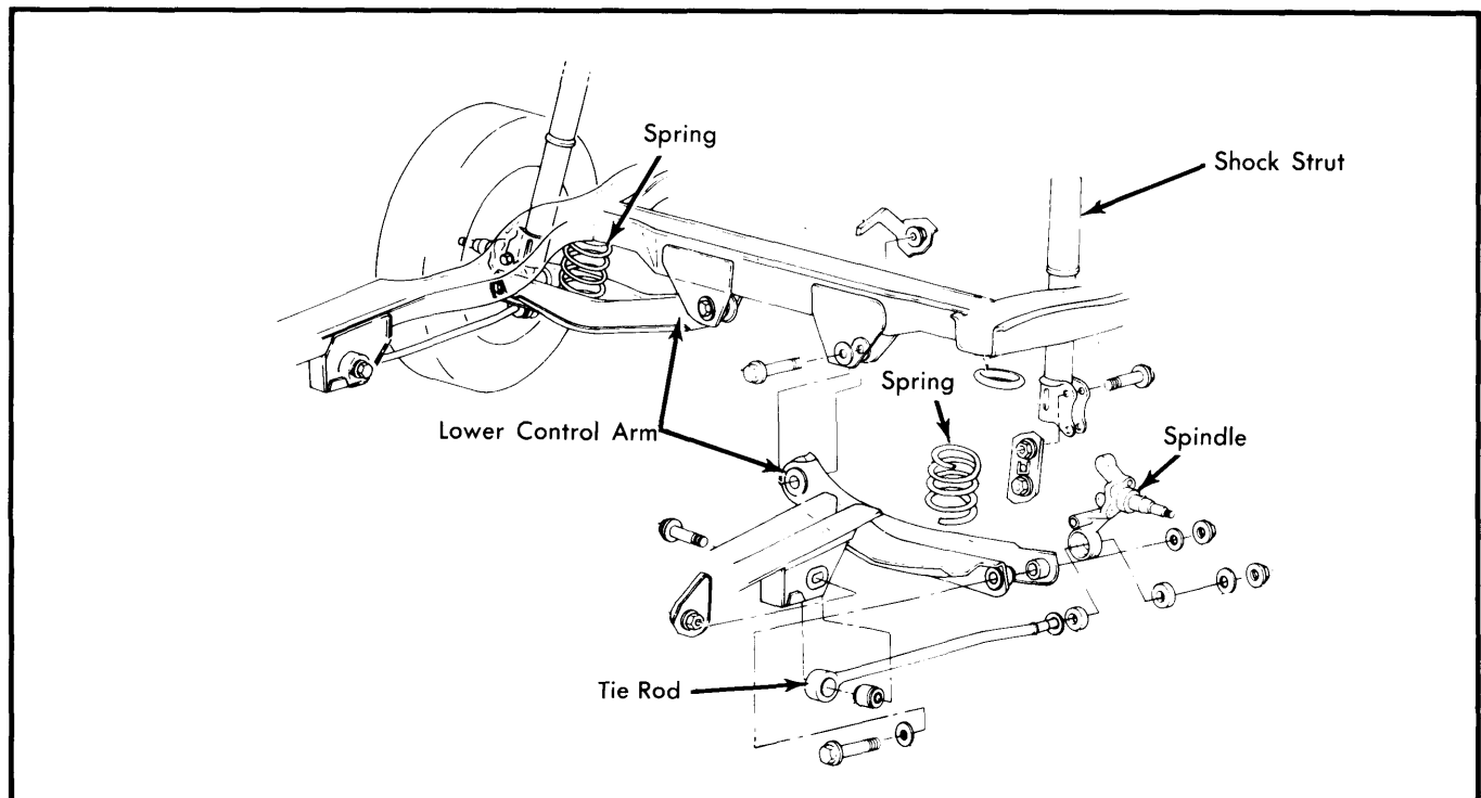
Fig. 1 Rear Suspension Assembly, Escort and Lynx
