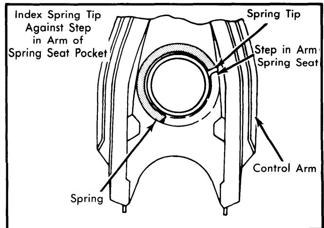
Fig. 2 Index Location for Rear Spring
