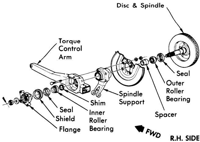
Fig. 3 Spindle Assembly
