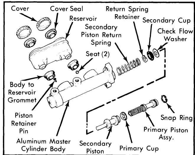
Fig. 7 Chrysler Corp. Aluminum Body Master Cylinder
