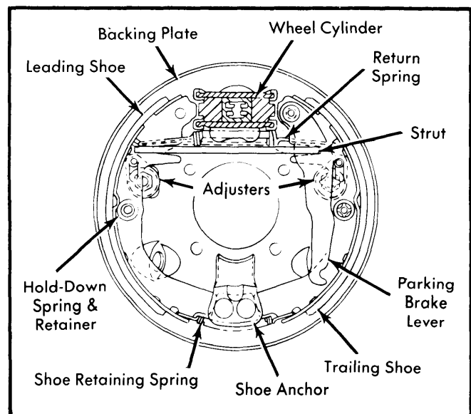
Fig. 2 Brake Assembly
