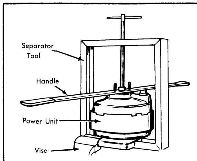
Fig. 2 Separating Front and Rear Housings Showing Separator Tool and Spanner Handle
