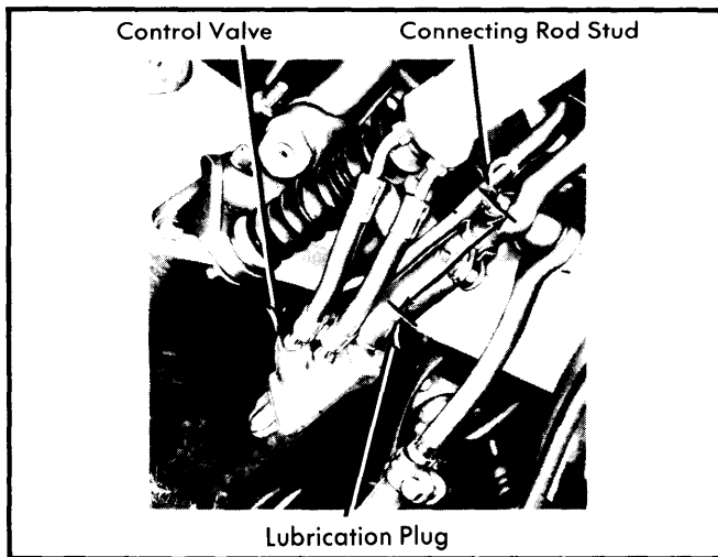
Fig. 3 Control Valve Installation Measurement
