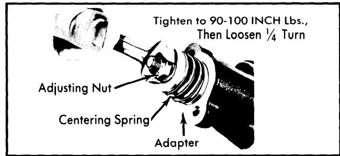
Fig. 1 Adjusting Centering Spring
