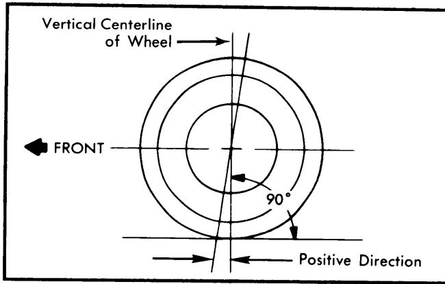
Fig. 4 Determining Caster Angle
