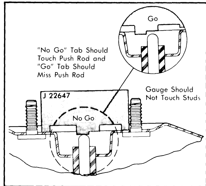
Fig. 2 Using "Go-No Go" Push Rod Gauge to Measure Height of Push Rod
