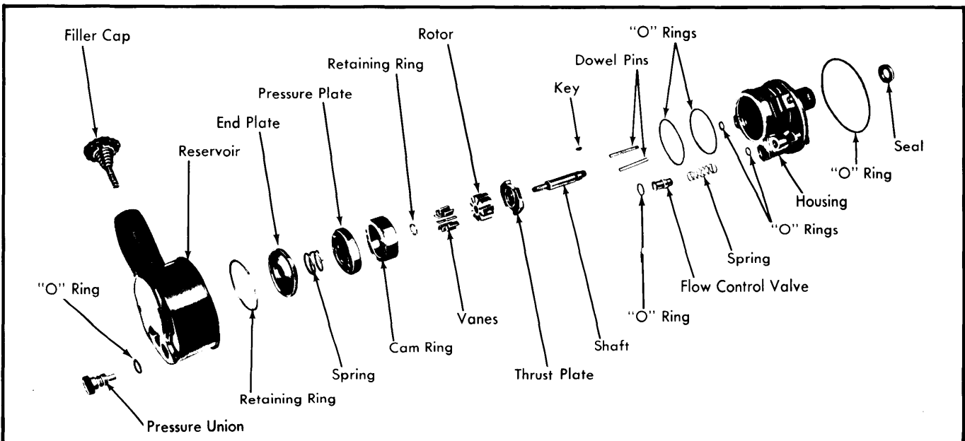
Fig. 1 Saginaw Vane Power Steering Pump
