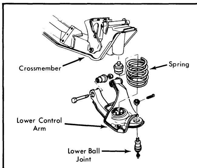
Fig. 2 View Showing Correct Positioning of Coil Spring
