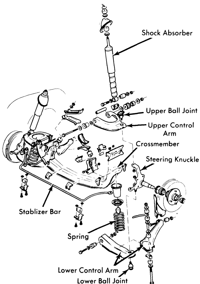
Fig. 1 Exploded View of Chevette Front Suspension Assembly
