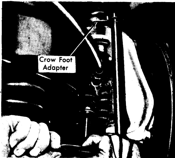
Fig. 15 Camber Adjustment Except Eldorado & Seville
