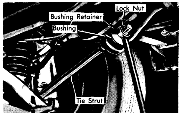
Fig. 14 Caster Adjustment Except Eldorado & Seville
