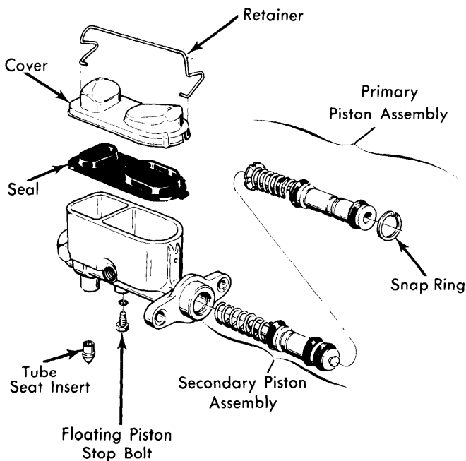
Fig. 3 Bendix Master Cylinder (Ford Motor Co. Shown)
