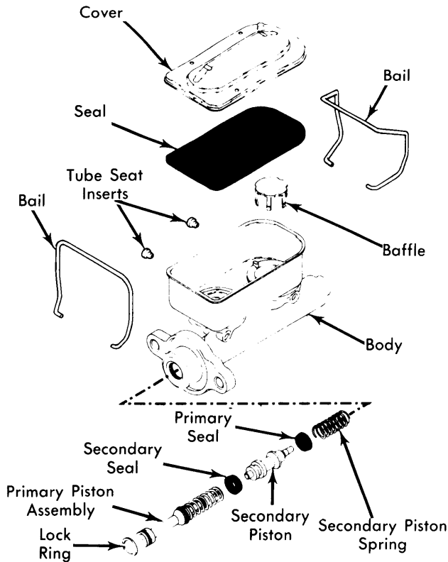
Fig. 5 Common Reservoir Power Brake Master Cylinder (General Motors Shown)
