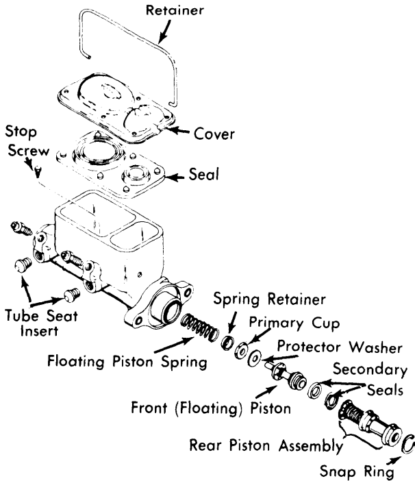
Fig. 2 Typical Delco-Moraine Dual Reservoir Master Cylinder (General Motors Shown)
