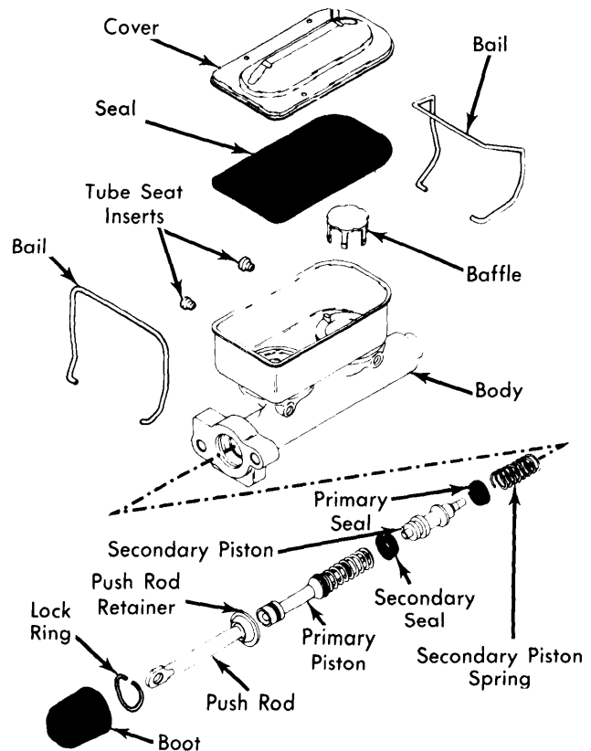
Fig. 4 Common Reservoir Manual Brake Master Cylinder (General Motors Shown)
