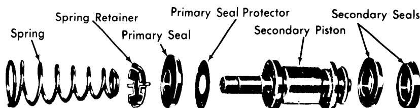
Fig. 7 Exploded View of Secondary Piston Assembly
