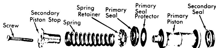
Fig. 6 Exploded View of Primary Piston Assembly
