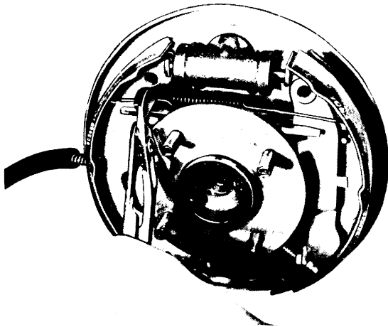
Fig. 6 Pull Back Spring Position
