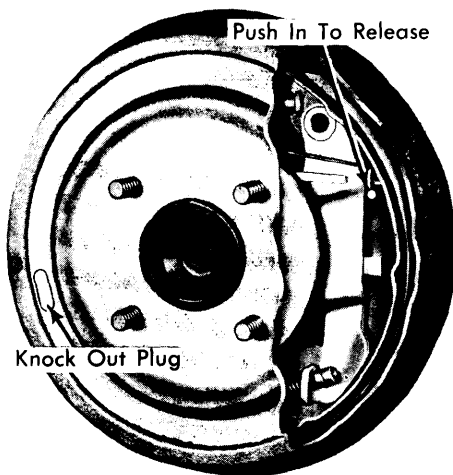
Fig. 1 Brake Drum Release Provision
