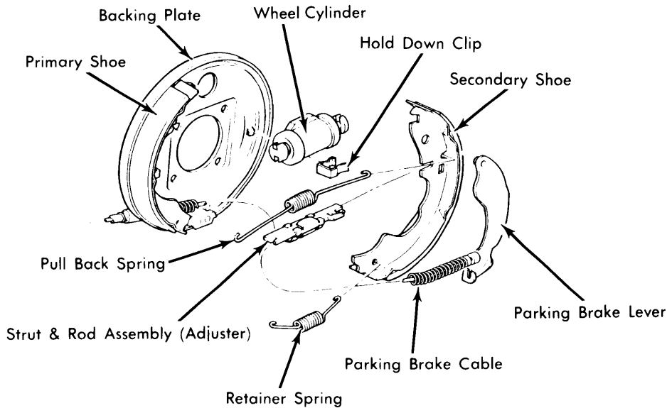
Fig. 7 Exploded View of Rear Brake Assembly
