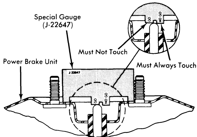
Fig. 4 Chevrolet Push Rod Gauging Method with Special "GO-NO GO" Gauge J-22647
