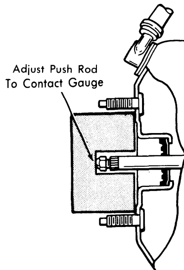
Fig. 2 Measuring Push Rod Height (Ford Motor Co.)
