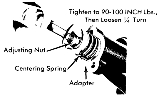
Fig. 1 Adjusting Centering Spring
