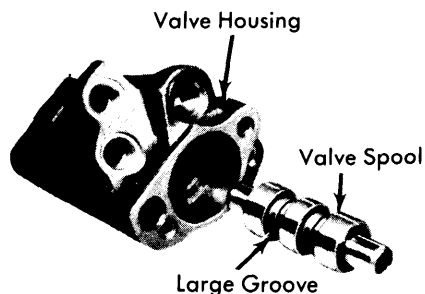
Fig. 5 Valve Spool Installation
