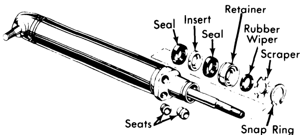
Fig. 4 Power Cylinder Assembly
