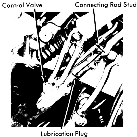
Fig. 3 Control Valve Installation Measurement
