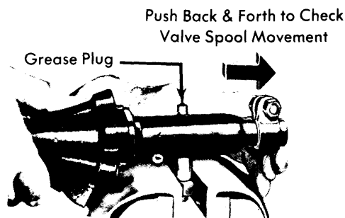
Fig. 6 Checking Valve Spool Movement
