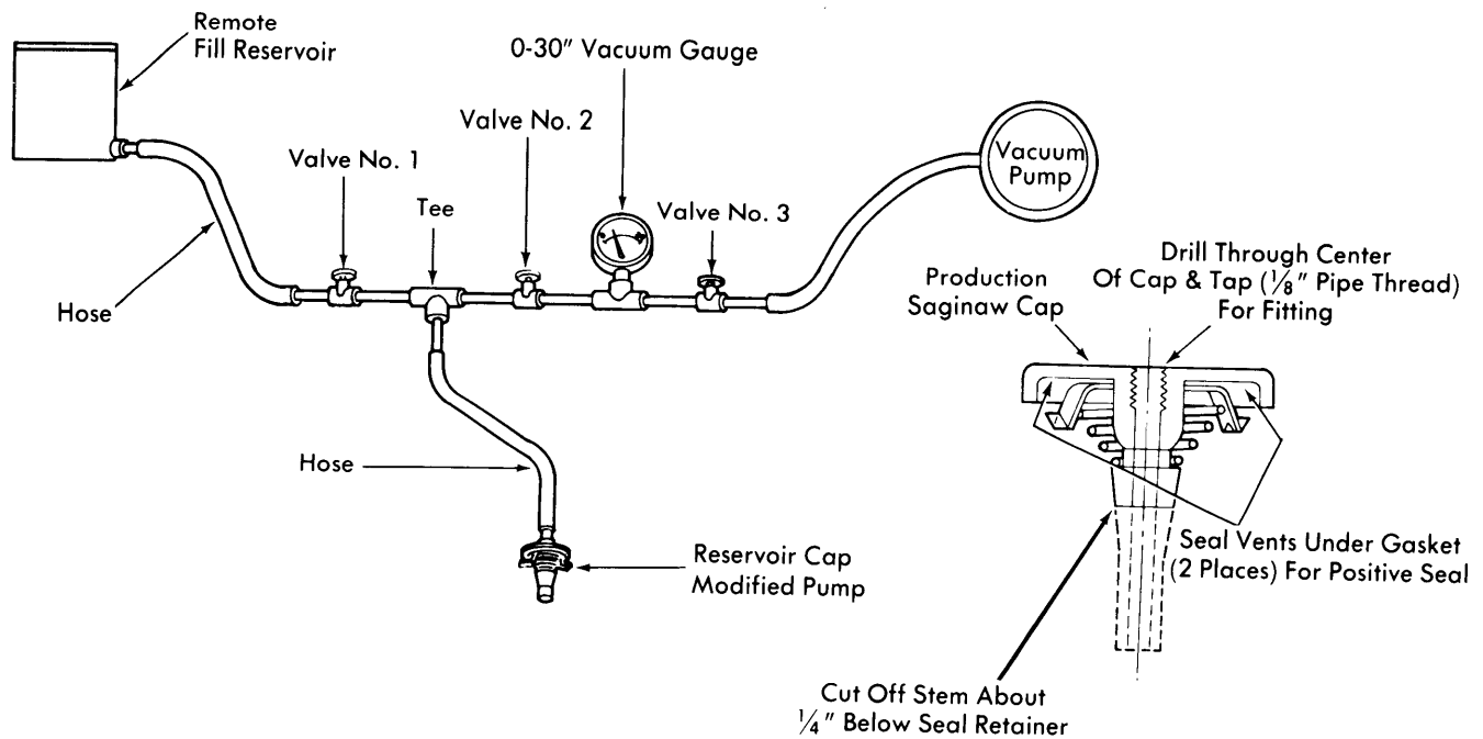
Fig. 2 Vacuum Fill System
