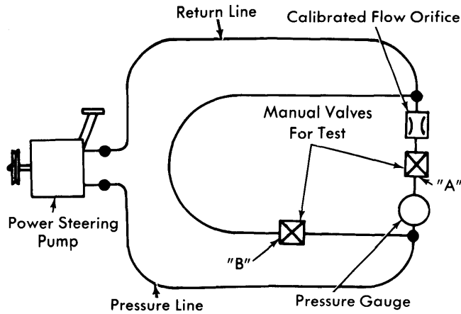
Fig. 4 Power Steering Pump Test Schematic
