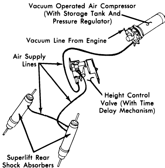
Fig. 1 Automatic Leveling System
