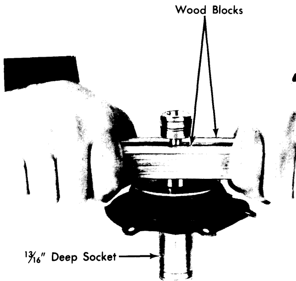
Fig. 4 Installing Diaphragm Retainer
