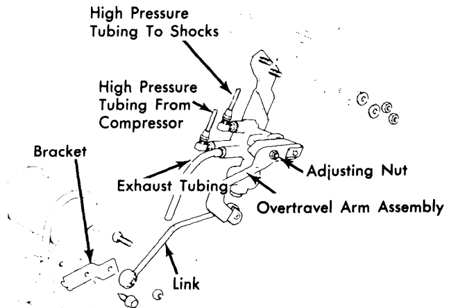
Fig. 3 Height Control Valve
