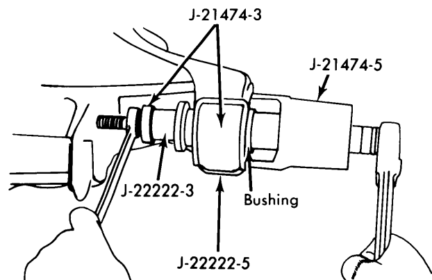
Fig. 4 Lower Control Arm Bushing Removal
