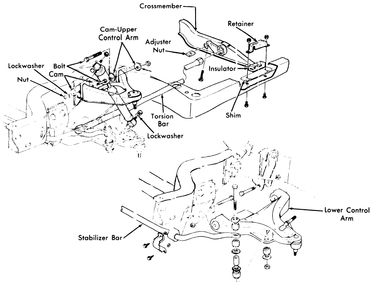
Fig. 3 Eldorado and Toronado Front Suspension Assembly
