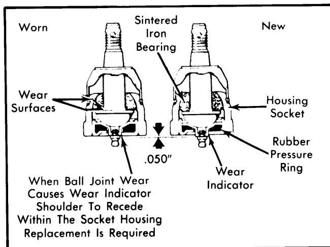
Fig. 1 G.M. Lower Ball Joint Wear Indicator
