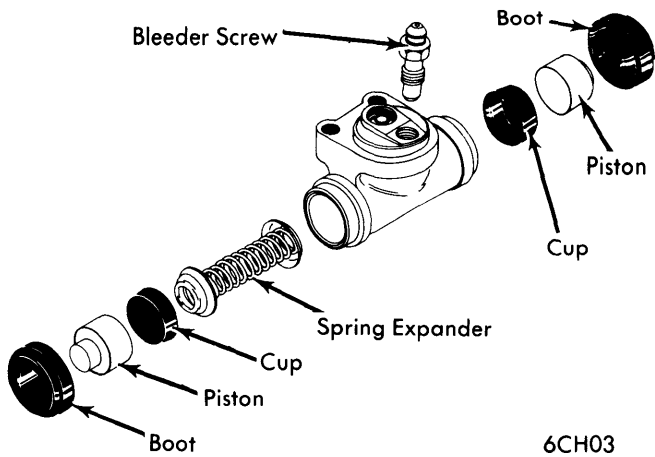
WHEEL CYLINDER DISASSEMBLED
