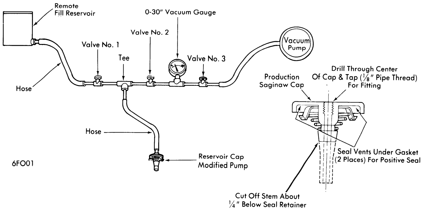
VACUUM FILL SYSTEM
