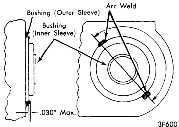
3F6001 LOWER CONTROL ARM BUSHING INSTALLATION (TACK WELD)
