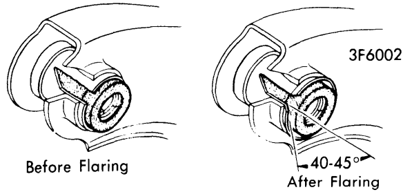
LOWER CONTROL ARM BUSHING INSTALLATION (FLARING)
