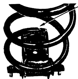
Lower Coil End Must Butt Against Formed Shoulder In Spring Seat
