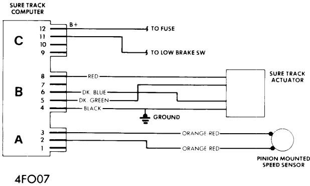
FORD SURE TRACK WIRING DIAGRAM
