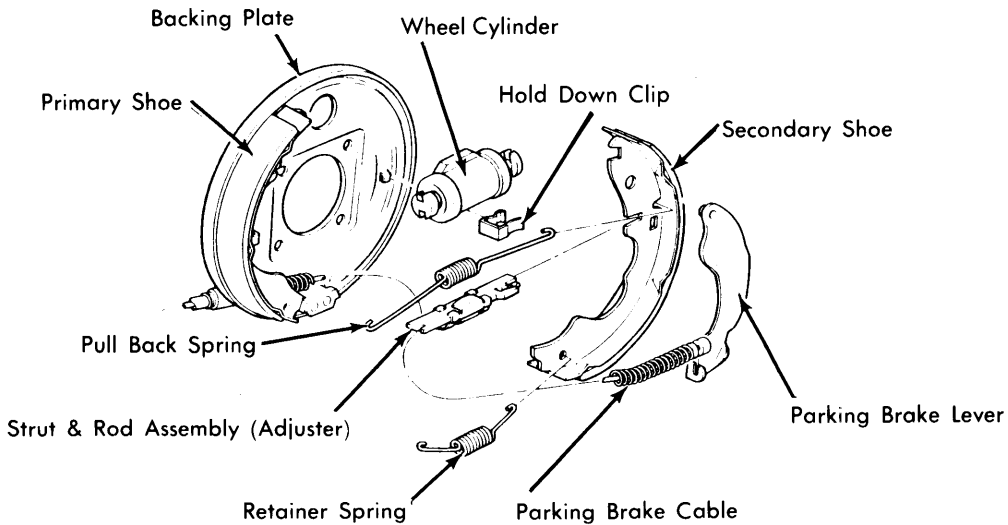
VEGA REAR BRAKE ASSEMBLY
