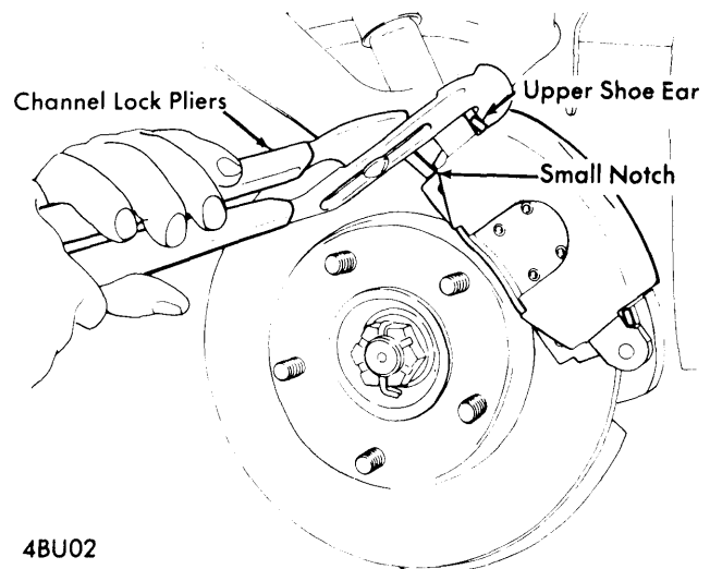
CLINCHING OUTBOARD SHOE
