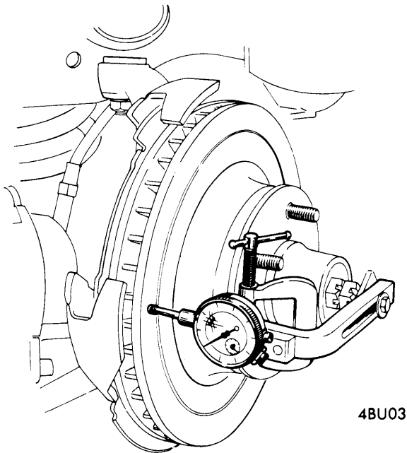
CHECKING LATERAL RUNOUT (TYPICAL)
