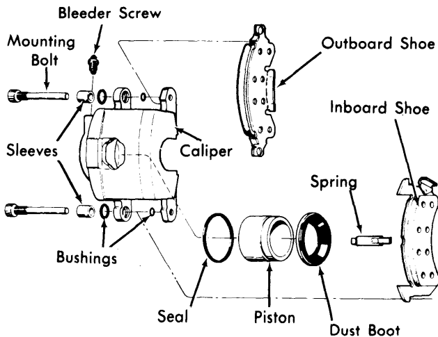
CALIPER ASSEMBLY
