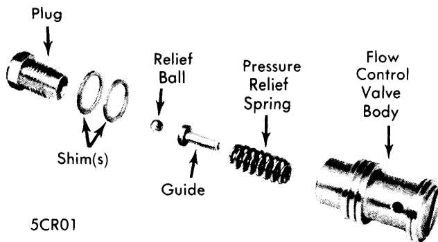
FLOW CONTROL VALVE
