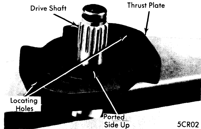
INSTALLING THRUST PLATE
