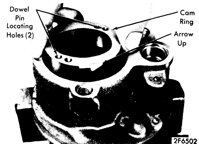
INSTALLING CAM RING
