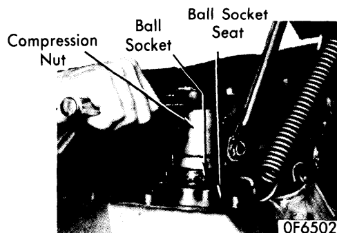
INSTALLING SPRING COMPRESSOR TOOL IN UPPER SPRING OPENING
