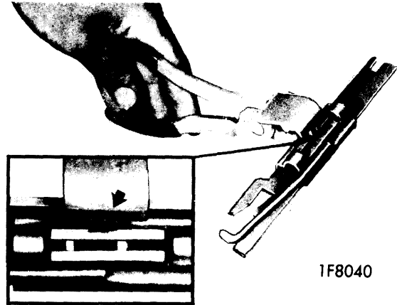
RELEASING ADJUSTER LOCKS
