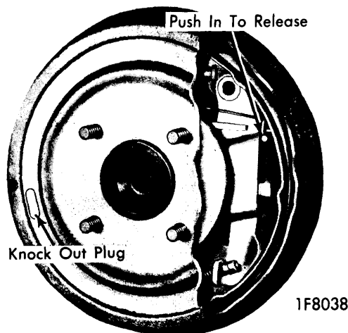
BRAKE DRUM RELEASE PROVISION
