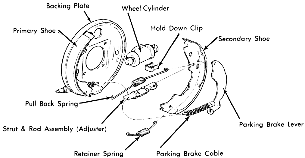
VEGA REAR BRAKE ASSEMBLY
