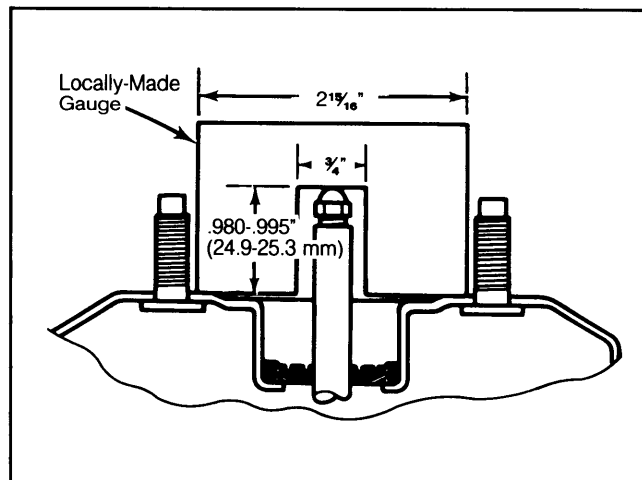
Ford models are checked with locally-made gauge.
