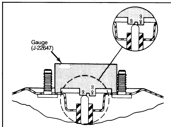
Chevrolet and GMC are checked with J-22647 gauge.
