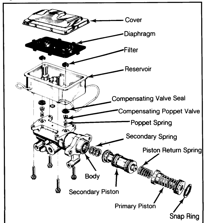
Fig. 1: Exploded View of Bendix Mini-Master Cylinder
