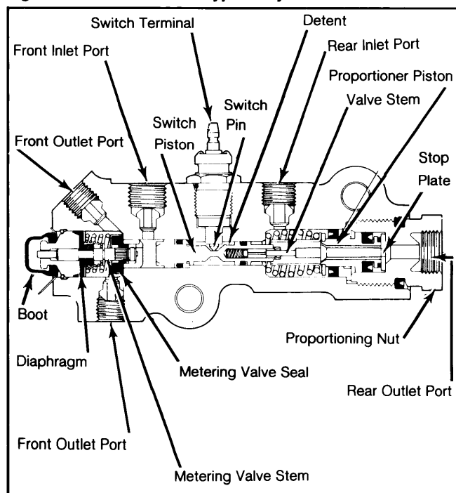
Fig. 1: Sectional View of Typical Hydraulic Control Valve
