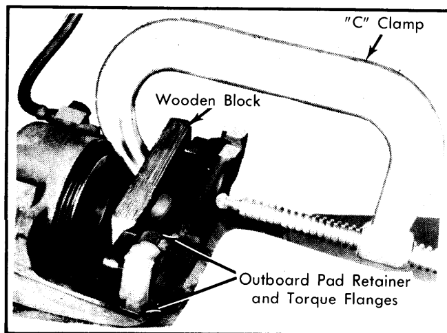
Fig. 3 Installation of Outboard Pad and Liner
