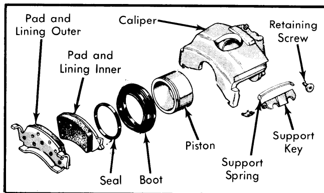
Fig. 2 Exploded View of Bendix Single Piston Disc Brake Caliper
