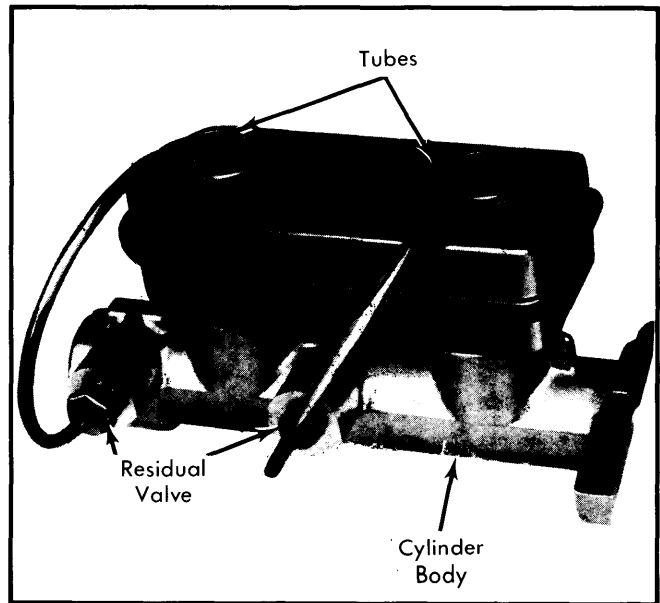
Fig. 3 Master Cylinder Bleeding Procedure
