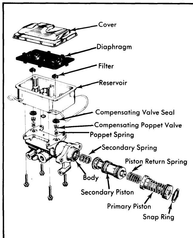
Fig. 1 Exploded View of Bendix Mini-Master Cylinder
