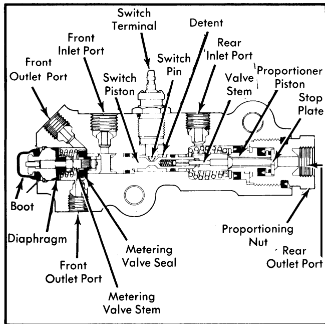
Fig. 1 Sectional View of Typical Hydraulic Control Valve
