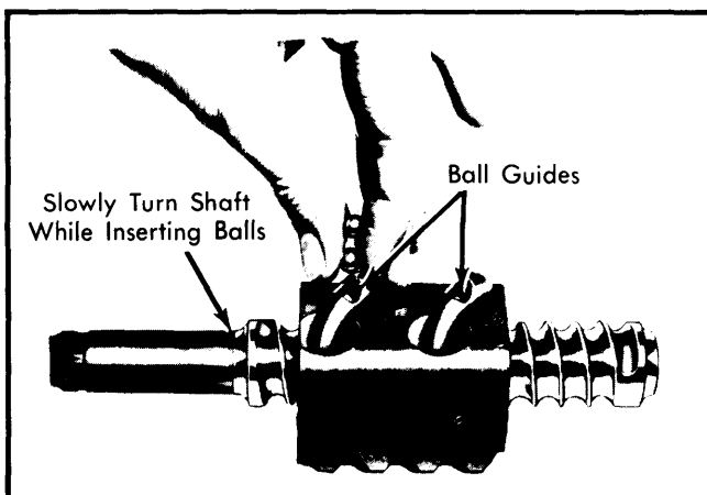
Fig. 6 Filling Ball Circuits Through Holes in Ball Guides
