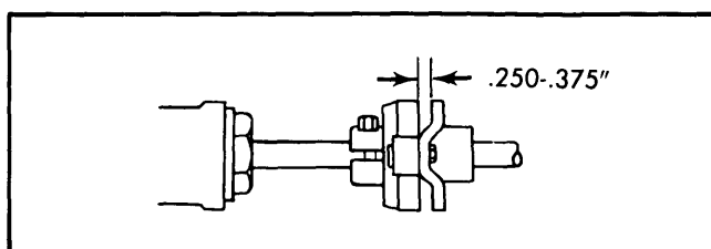
Fig. 3 Adjusting Flexible Coupling for All General Motors Models
