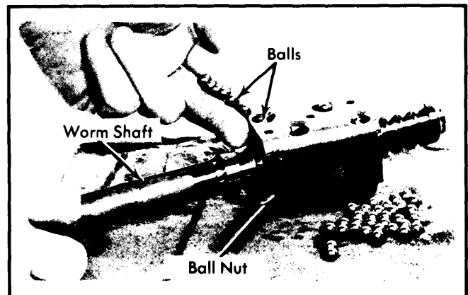
Fig. 7 Filling Ball Circuits Through Holes in Ball Nut
