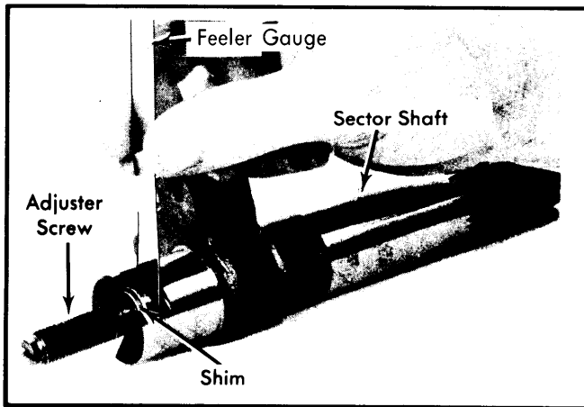
Fig. 8 Checking Lash Adjuster Clearance
