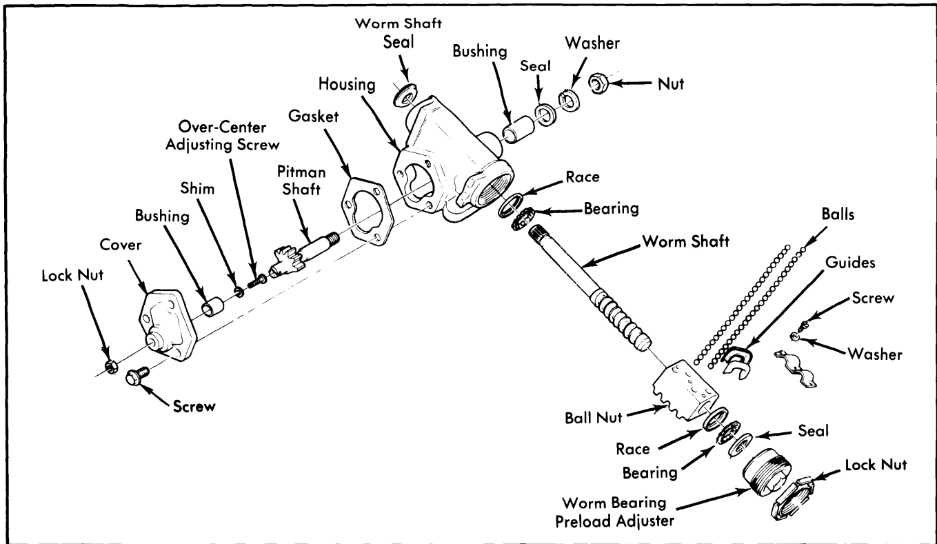
Fig. 5 Exploded View of Recirculating Ball Steering Gear (General Motors Model Shown)
