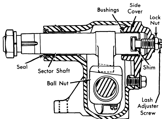
Fig. 2 Cross Section of Steering Gear
