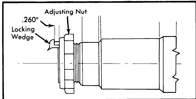
Fig. 1 Installing Locking Wedge Chrysler Corp. and Ford E250 and E350 Models
